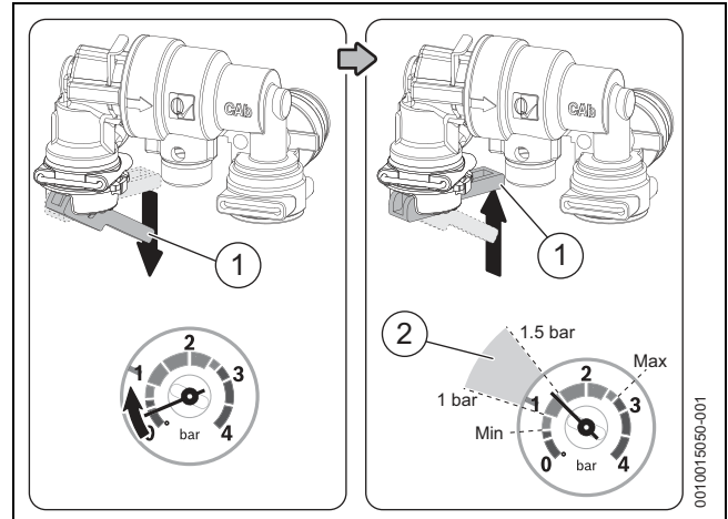
Fig. 5 Keyless filling link
