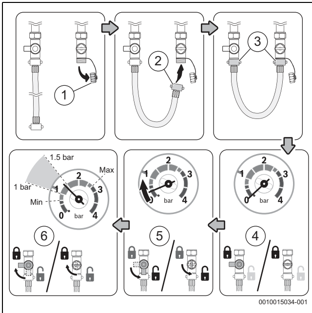
Fig. 4 External filling loop
