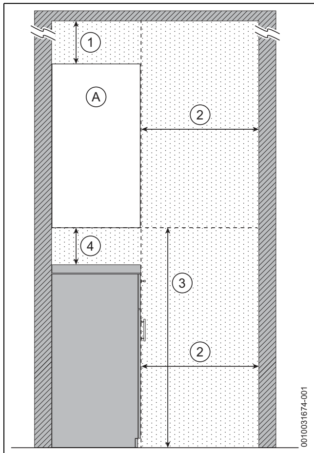
Fig. 10 Reduced front maintenance clearances - Side view
