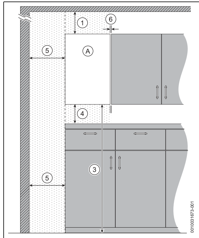
Fig. 11 Reduced front maintenance clearances - Front view
